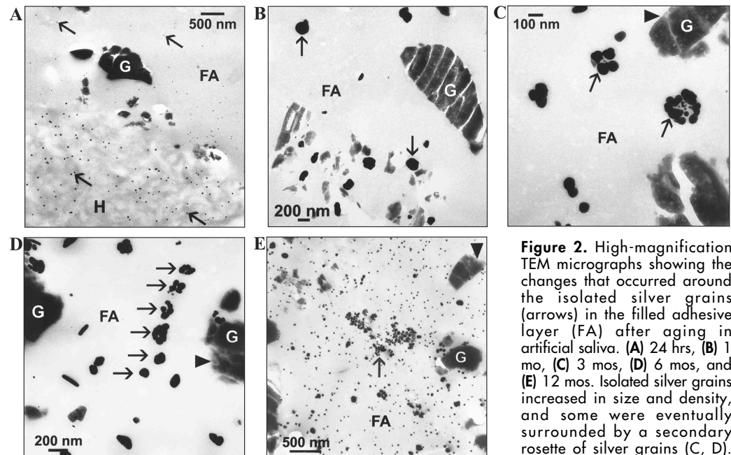
Figure 2. High-magnification TEM micrographs showing the changes that occurred around the isolated silver grains (arrows) in the filled adhesive layer (FA) after aging in artificial saliva. (A) 24 hrs, (B) 1 mo, (C) 3 mos, (D) 6 mos, and (E) 12 mos. Isolated silver grains increased in size and density, and some were eventually surrounded by a secondary rosette of silver grains (C, D). The precursors of water-filled channels ( i.e. , water trees) that could be seen at 6 mos were attributed to the increase in density of these rosettes of silver grains. Frank water trees were evident at 12 mos (E). A siliceous hydrogel layer (arrowheads) could also be observed along the periphery of the fluoroaluminosilicate glass fillers (G) beginning at 3 mos.
