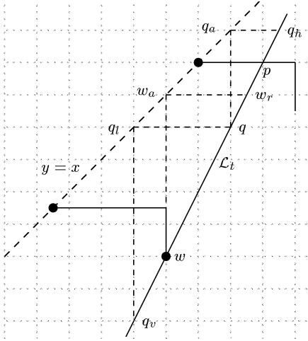
Figure 4: The position of the points in \text{Slave}(q) .
