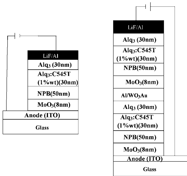
FIG. 1. Schematic diagram of one-unit and tandem devices.
