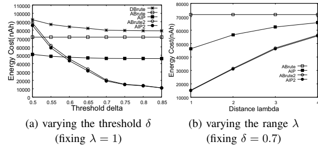
Fig. 4. Energy cost of protocols, COR data, at N = 1024
