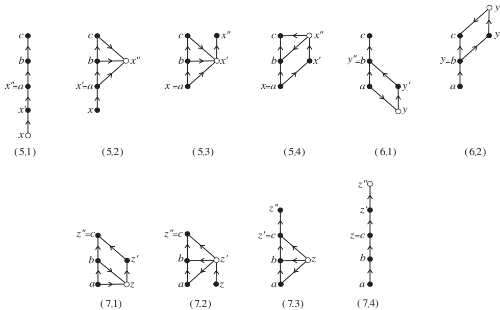
FIG. 3. Possible configurations of triangles xx'x''x , yy'y''y , and zz'z''z .
