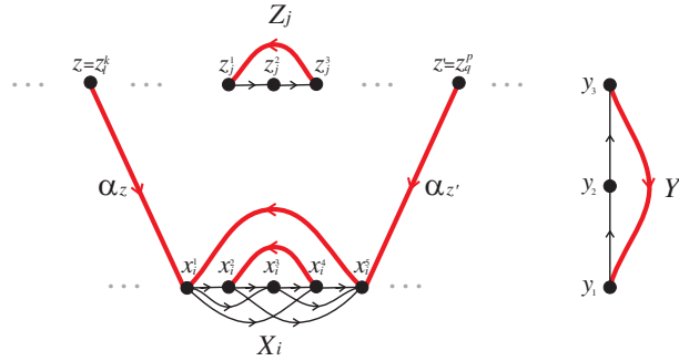
FIG. 4. An illustration of constructions (i)–(iv), where c_l^k = \lambda_i and c_q^p = \bar{\lambda}_i .
