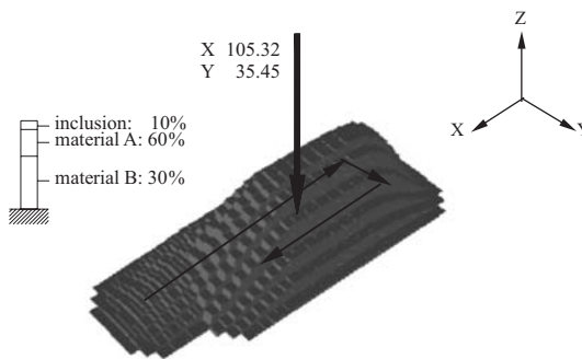
Figure 5: The visualized simulation for the sprayed layer
